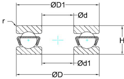
Miniature Thrust Bearing With Grooved Raceways
